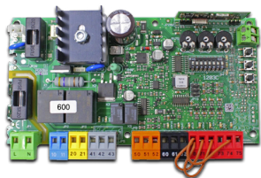
Hamal Control Board for BFT Deimos BTA 600
