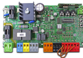
Hamal Control Board for BFT Deimos BTA 400
