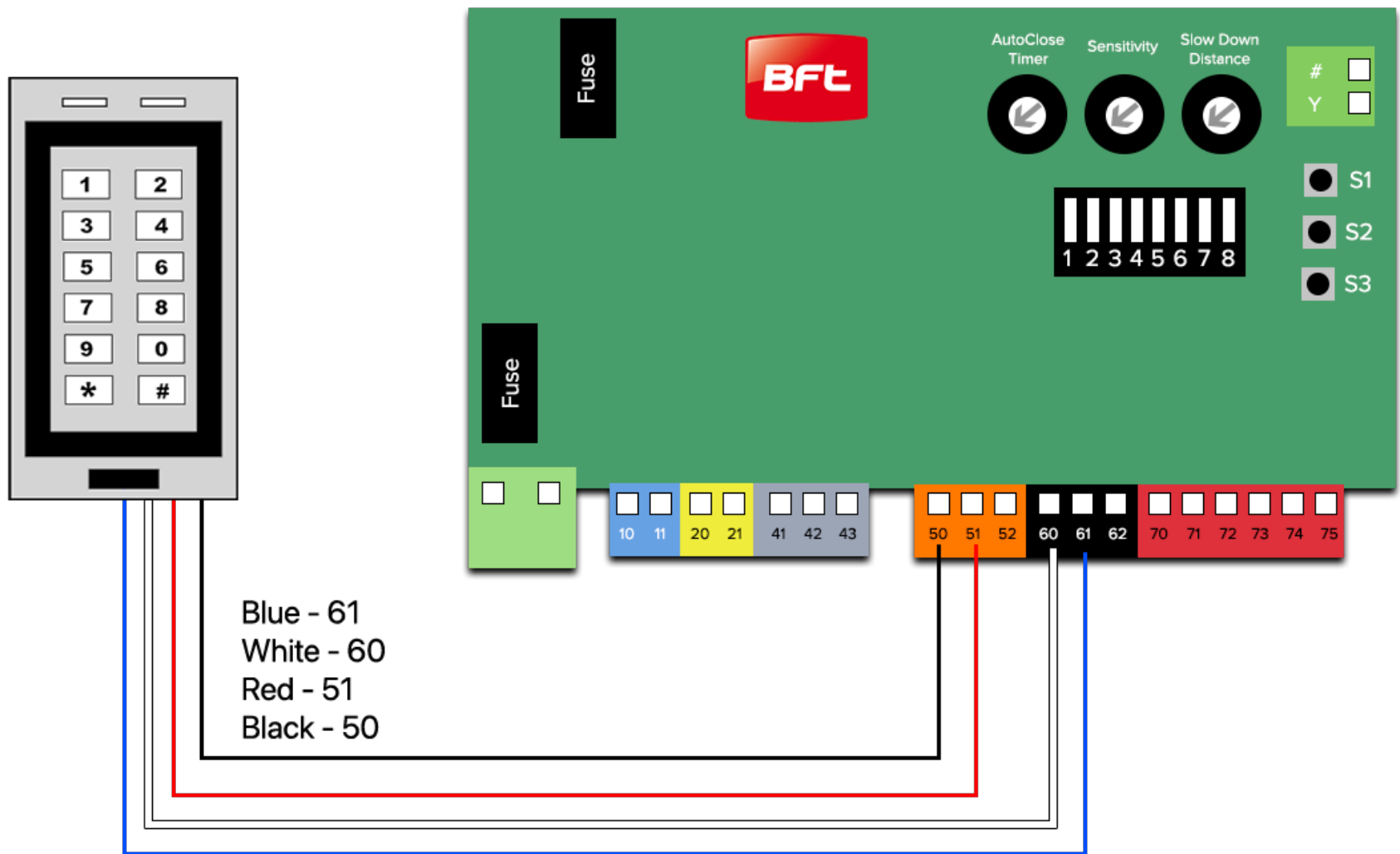
The old batch of ET270 (with white wire & blinking red light in idle state)
