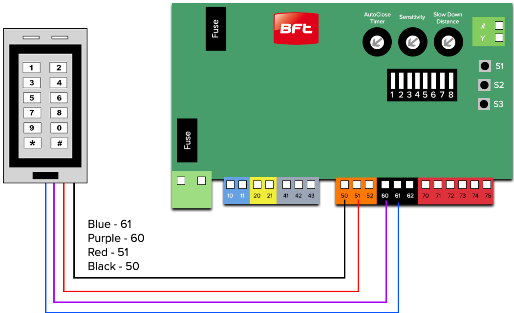
The new batch of ET270 (with purple wire & solid red light in idle state)
